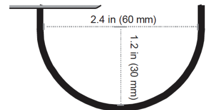
Figure 6. Minimum cable bend radius
