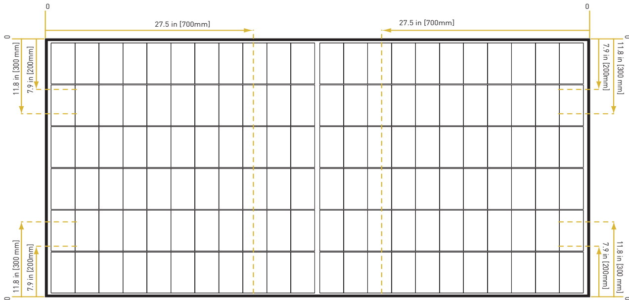
Figure 13. Clamping of EVPVxxxH Series modules with rails parallel to long side of the module
