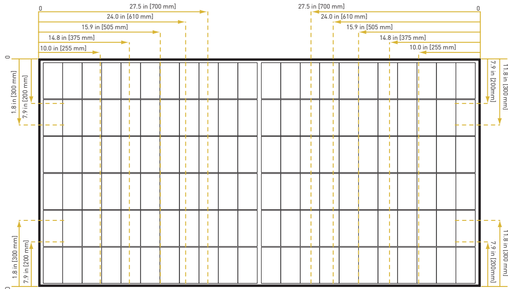
Figure 12. Clamping of EVPVxxxH Series modules with rails parallel to short side of the module
