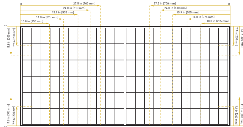
Figure 14. Clamping of EVPVxxxH Series modules using short rails
